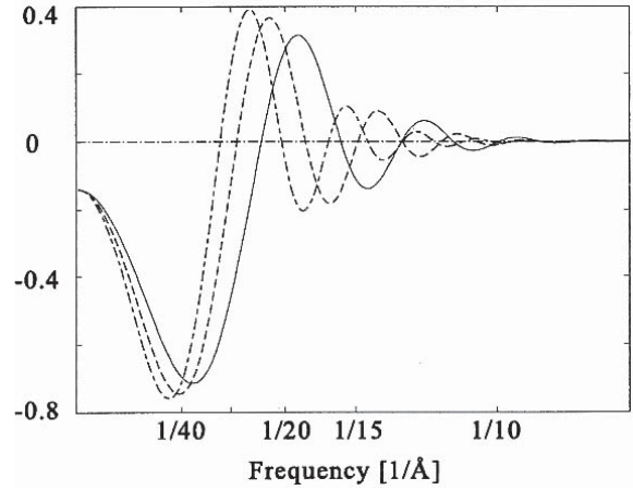
Figure 2. Theoretical contrast transfer function with envelope function effects for three defocus values: 1.5 \mu\text{m} (—), 2.0 \mu\text{m} (---), and 2.5 \mu\text{m} (-·-·-).
