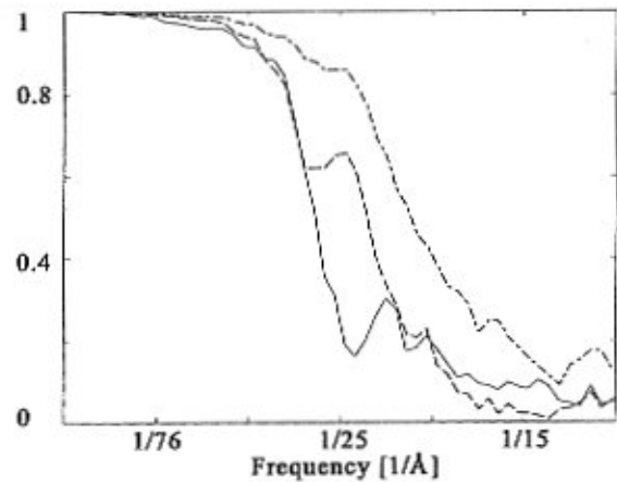
Figure 4. Resolution estimations using Fourier Shell Correlation curves for 1.5 \mu\text{m} (—), CTF-corrected (---), and CTF-corrected with positivity constraints (-·-·-) 3D reconstruction of the 70S E. coli ribosome.
